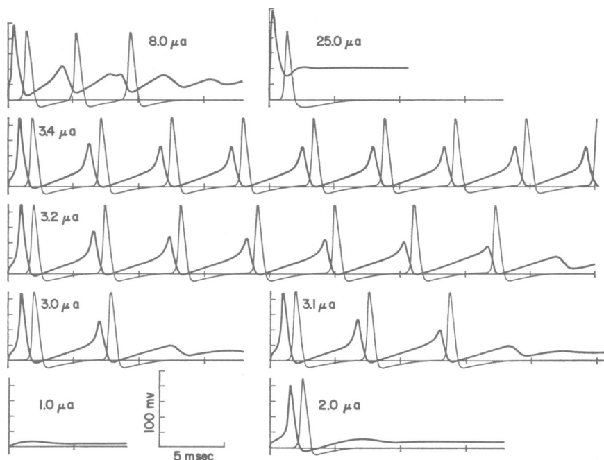
FIGURE 5 Response of the continuous axon to a steady stimulus of various intensities showing time course of the membrane potential V at x = 0 (heavy lines) and at x = 2 cm (lighter lines).
